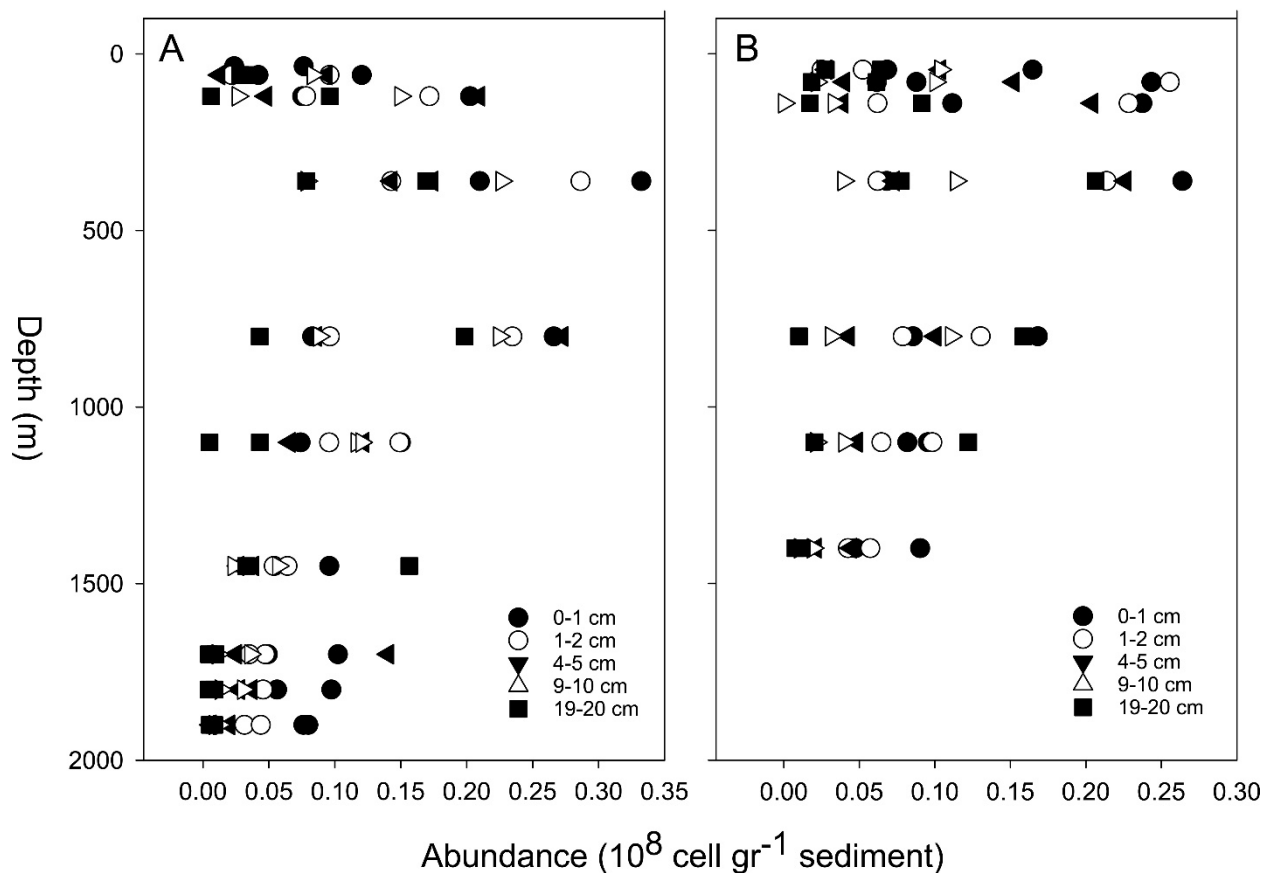
Prokaryote abundance in sediment profiles in Haifa (A) and Tel Aviv (B) sections
