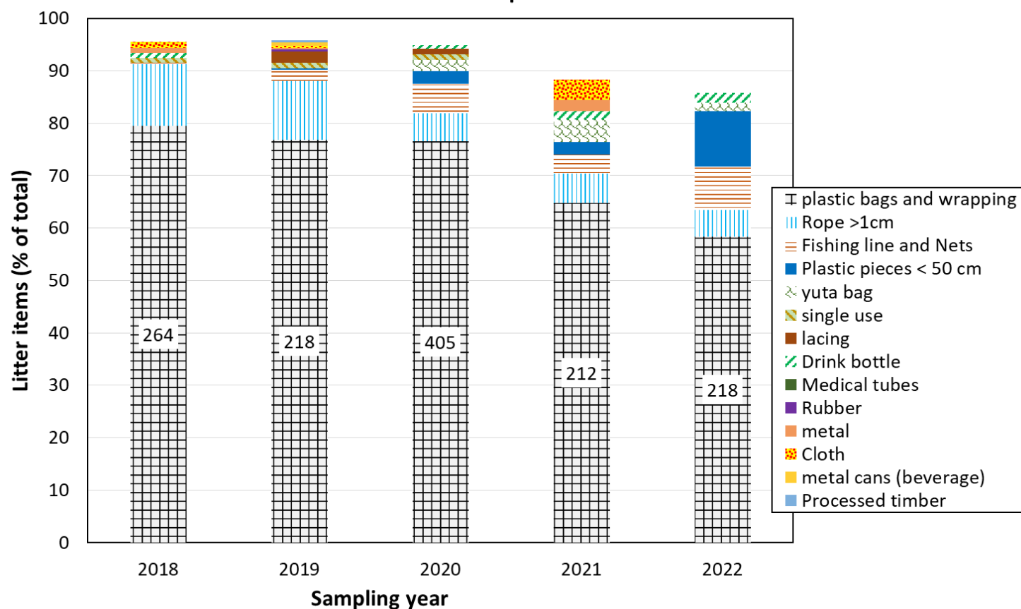
Coastal waters relative contribution of top ten bottom litter types >2.5cm found at 20-80m water depth
